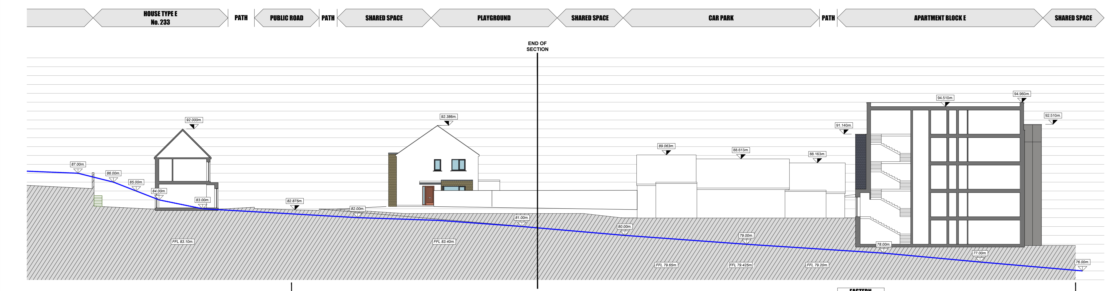
SITE SECTION J-J (2) SCALE 1:200
